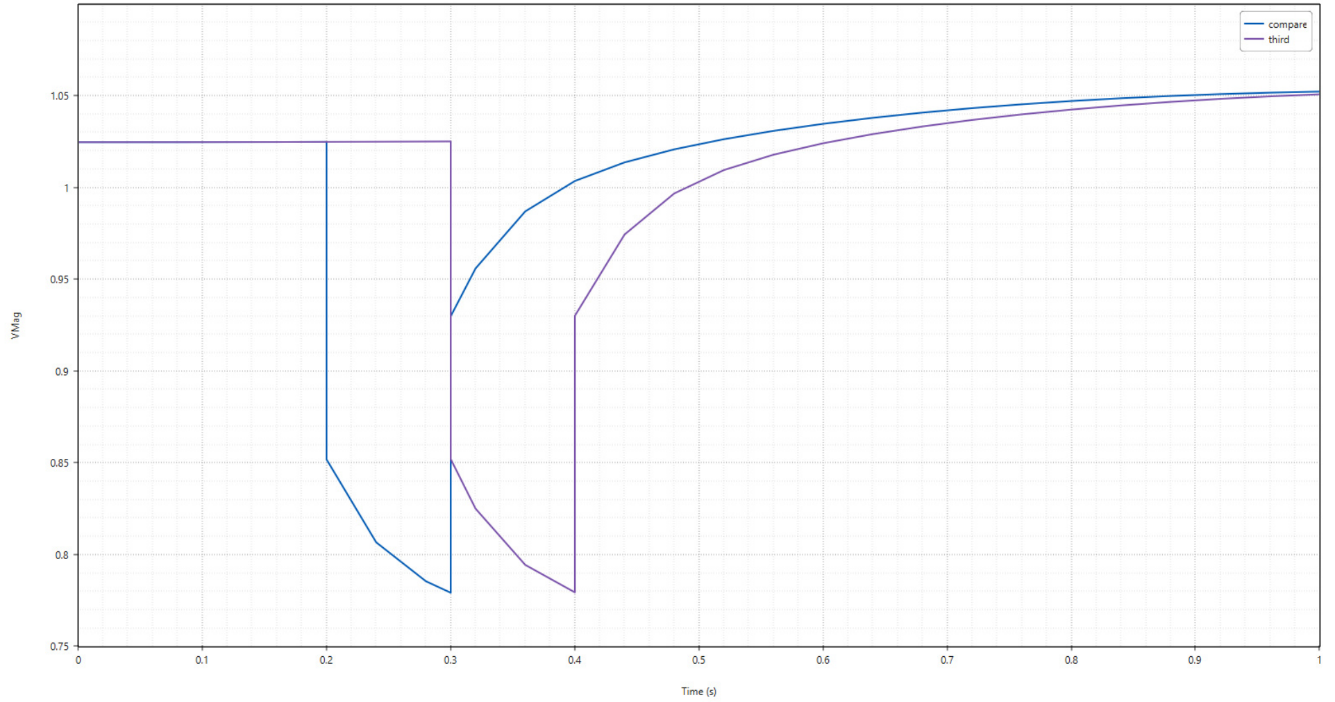
Busbars [5] - Voltage (PU)
