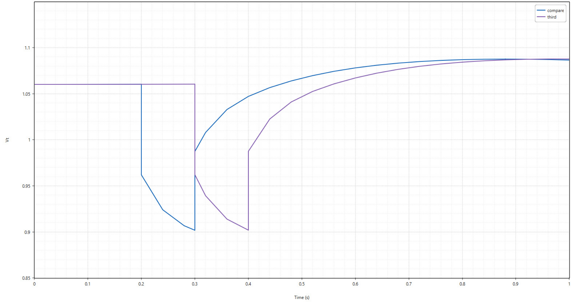
AVR controllers [1] - V_t
