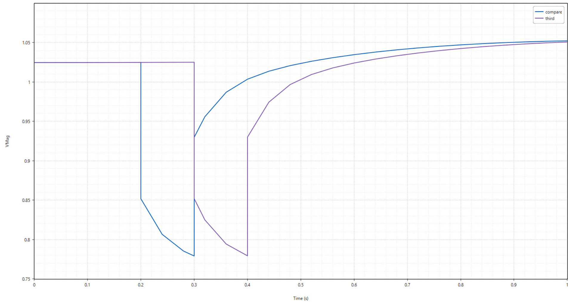
Busbars [5] - Voltage (PU)
