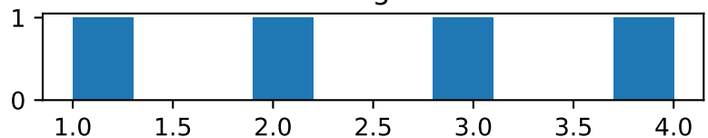
Histogram
