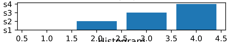
Bar graph
