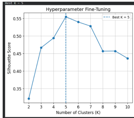
Finding Optimal K by hyperparameter tuning
