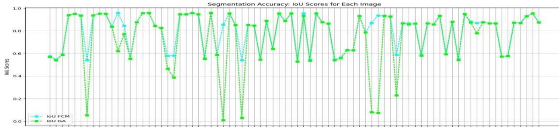
FIGURE 5. IoU Score for segmented images using FCM-GA [Source: Author].
