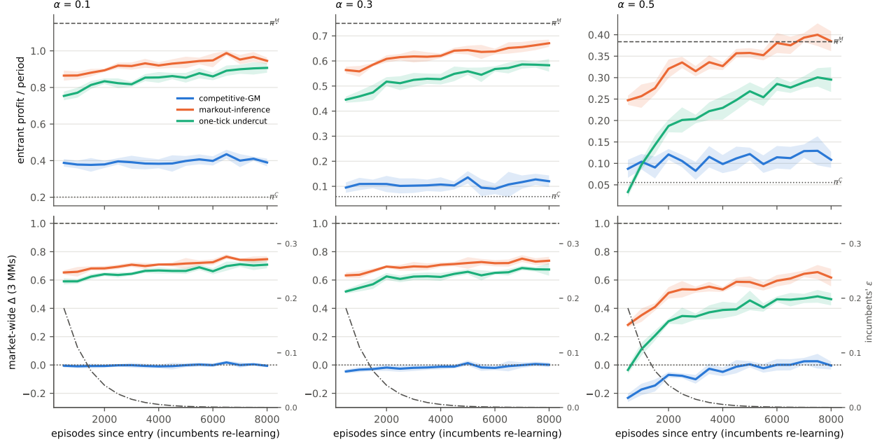
Figure 2: Entry against re-learning incumbents: entrant profit (top) and market-wide \Delta (bottom) over 8000 episodes, incumbents' \varepsilon on the twin axis. Dashed/dotted lines are per-incumbent \Pi^M , \Pi^C of the pre-entry market.
