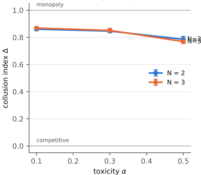
(a) Collusion index by toxicity and N
