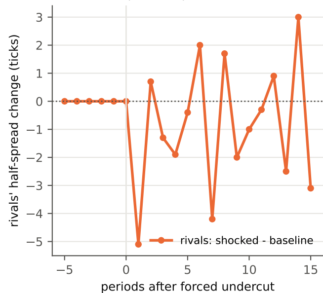
(c) Paired impulse response, \alpha=0.3 , N=2
