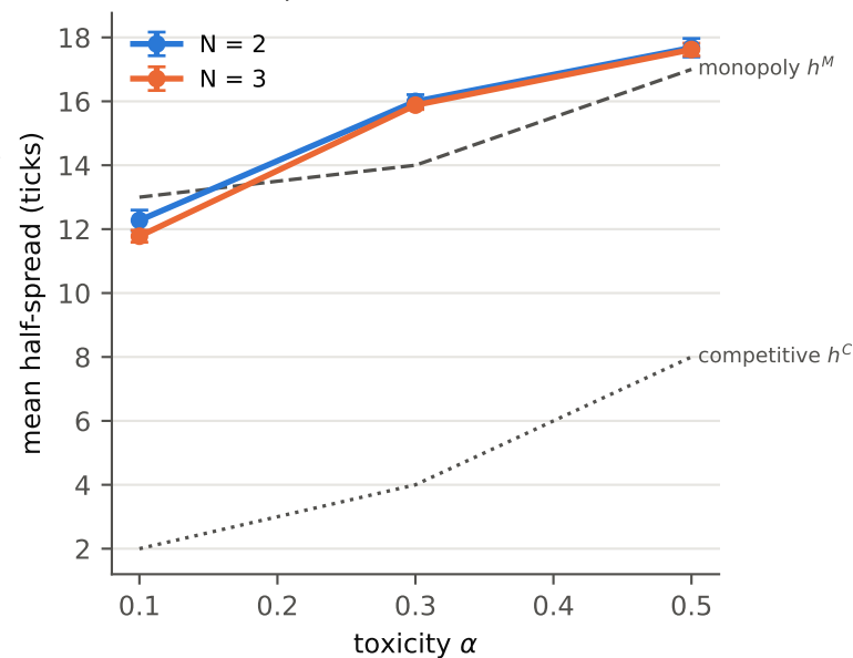
(b) Learned quotes vs exact benchmarks
