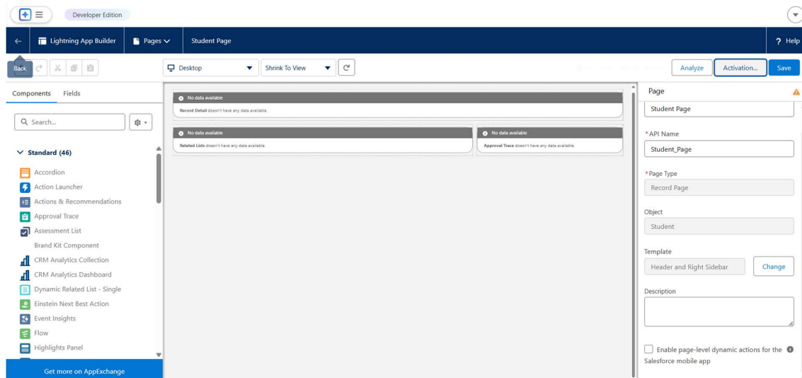
Fig 2.12: Lightning app builder
