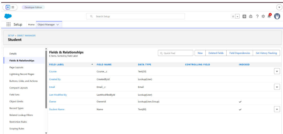
Fig 1.11 Attributes added
