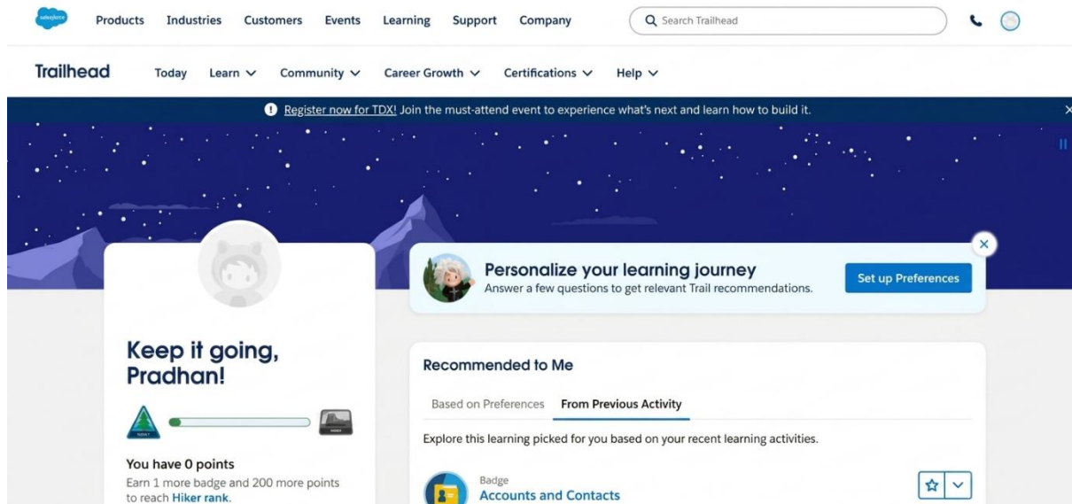
Fig 1.3 Trailhead Homepage
