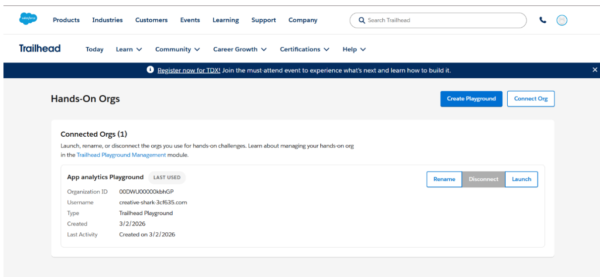
Fig 1.4 Playground Created
