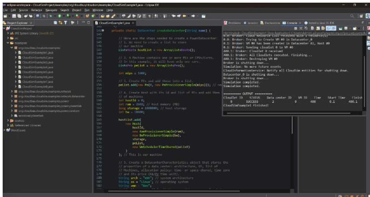
Fig 1.7 Simulation Successful
