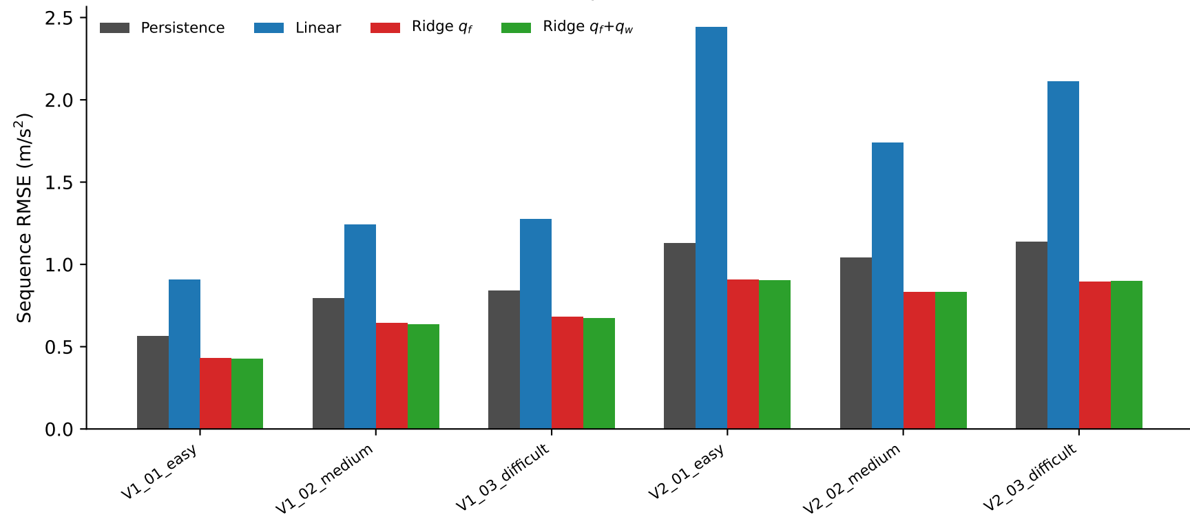
Within EuRoC: sequence multi-horizon RMSE
