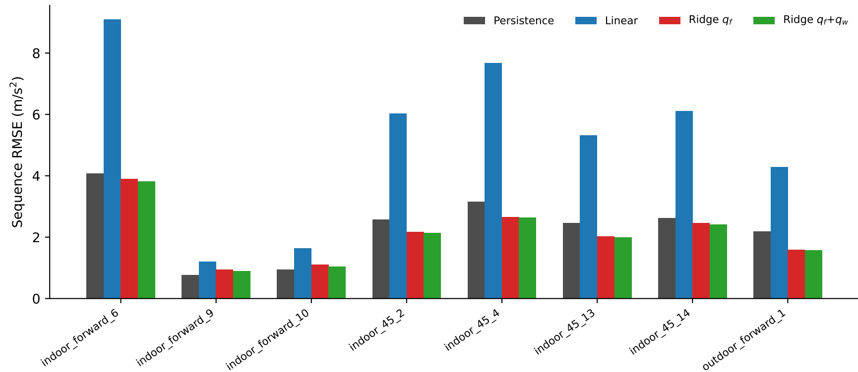
EuRoC → UZH zero-shot: sequence multi-horizon RMSE
