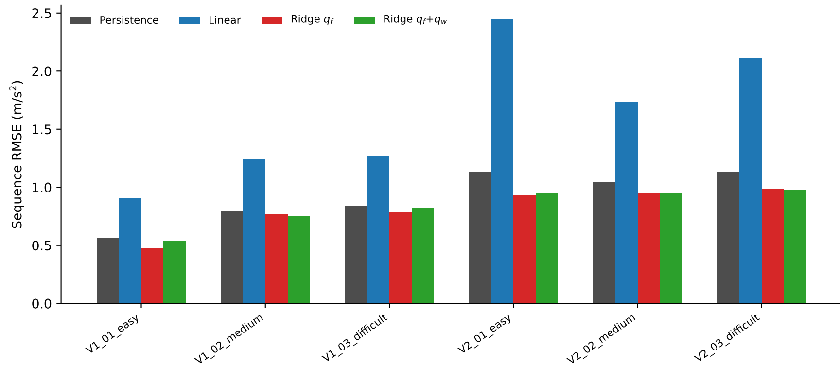
UZH → EuRoC zero-shot: sequence multi-horizon RMSE
