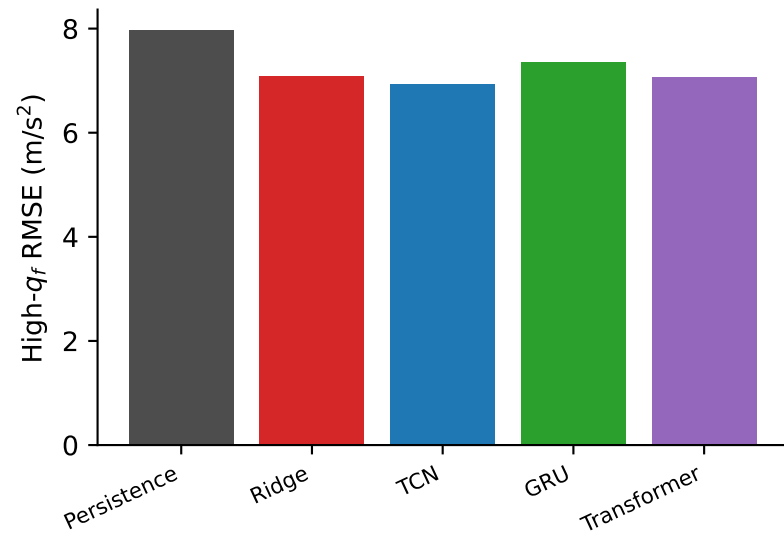
Within UZH-FPV
