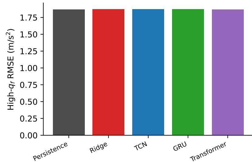
Within EuRoC
