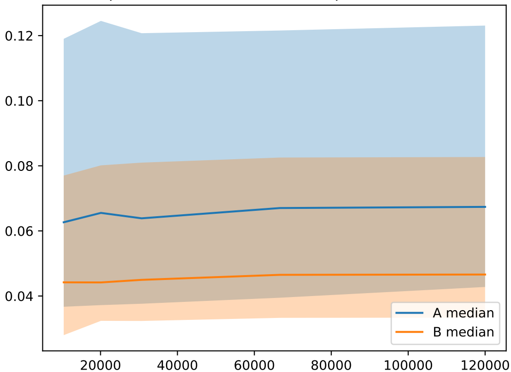
ICE Response Curve (Raw Q4 envelope) - 100062XXC08D
