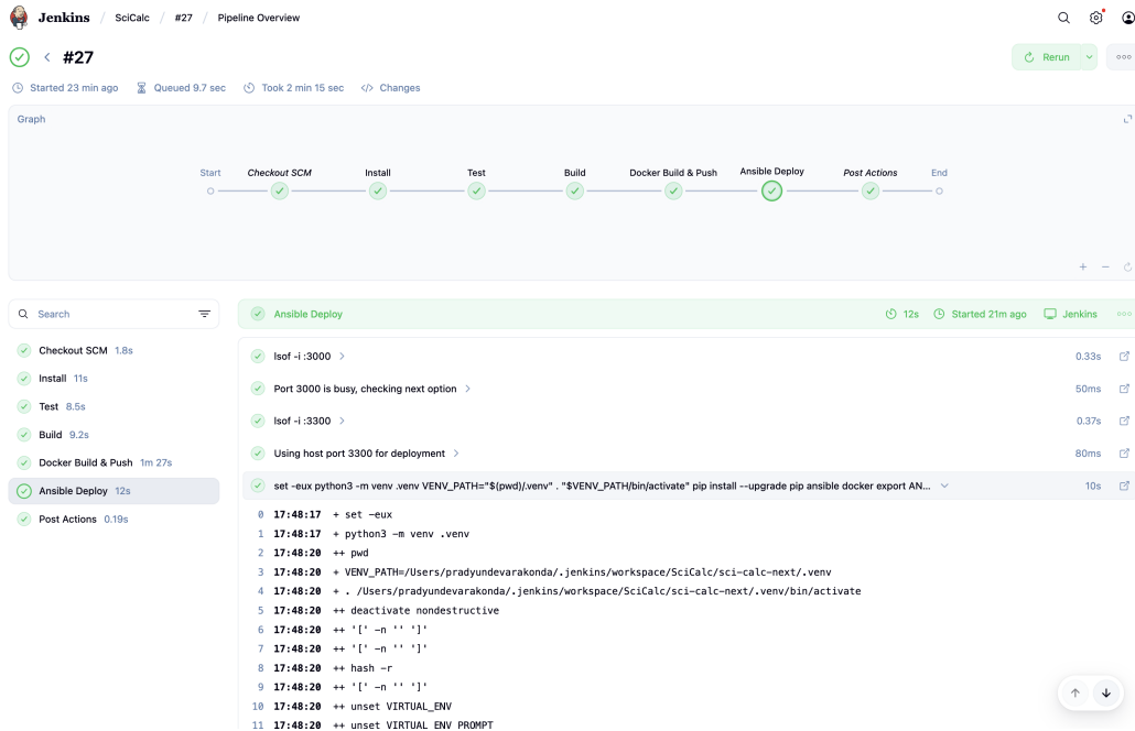
Figure 2: Jenkins pipeline stage view highlighting the passing Install, Test, Build, Docker, and Ansible stages.
