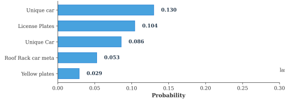
Figure 7: Interpretability analysis for Game 1 Round 9. The model identifies this location in West Africa through distinctive visual cues including unique vehicles and license plates, with balanced concept-spatial reasoning (gate 0.431). Top child concepts include “Unique car” and “License Plates”; parent concepts indicate “car_meta” and “landscape_savannah” categories.
