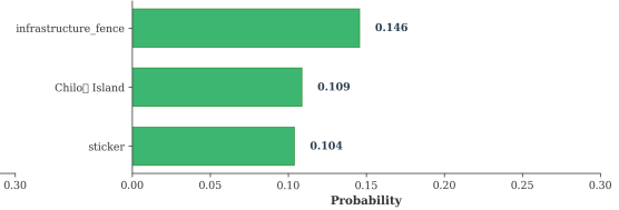
Figure 6: Interpretability analysis for Game 1 Round 1. This example demonstrates the model attending to architectural and infrastructure features for geolocation. The patch attention heatmap reveals focus on road geometry and built structures, while concept predictions capture semantic categories relevant to the predicted region.
