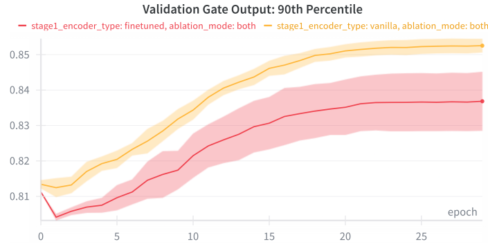
Figure 5: 90th percentile of learned gate values during validation over training epochs. Higher values indicate greater reliance on concept information versus spatial features. Both models converge to high gate values (0.83–0.86), with the vanilla variant showing slightly higher concept reliance than the finetuned variant.
