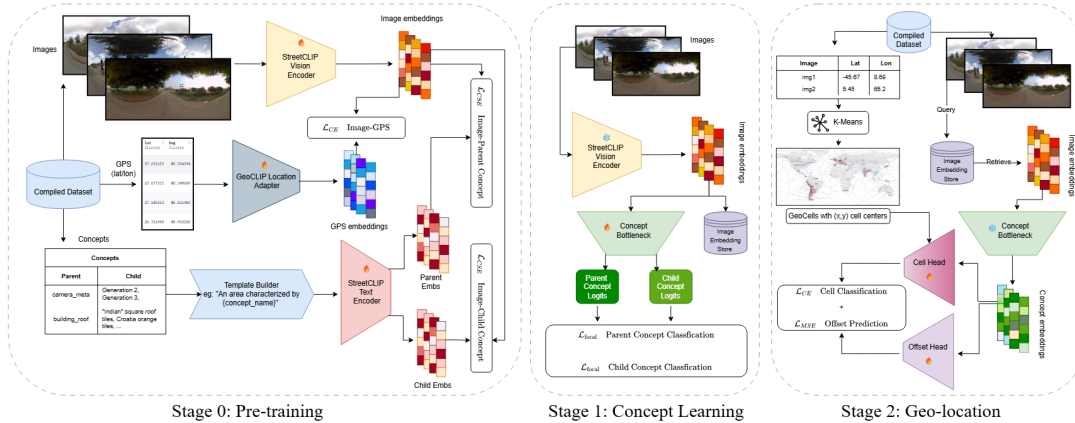
Figure 1: Three-stage architecture for concept-aware geolocation. Stage 0 performs domain contrastive pretraining to align image, GPS, and concept embeddings, with a GPS adapter (512d→768d) to align GeoCLIP location features with StreetCLIP image features. Stage 1 learns hierarchical concept classification through text-anchored prototypes with cosine similarity. Stage 2 predicts geographic coordinates via learned gated fusion: concept embeddings query image patches through cross-attention to extract spatial context, then a learned gate balances concept versus spatial information for each dimension.
