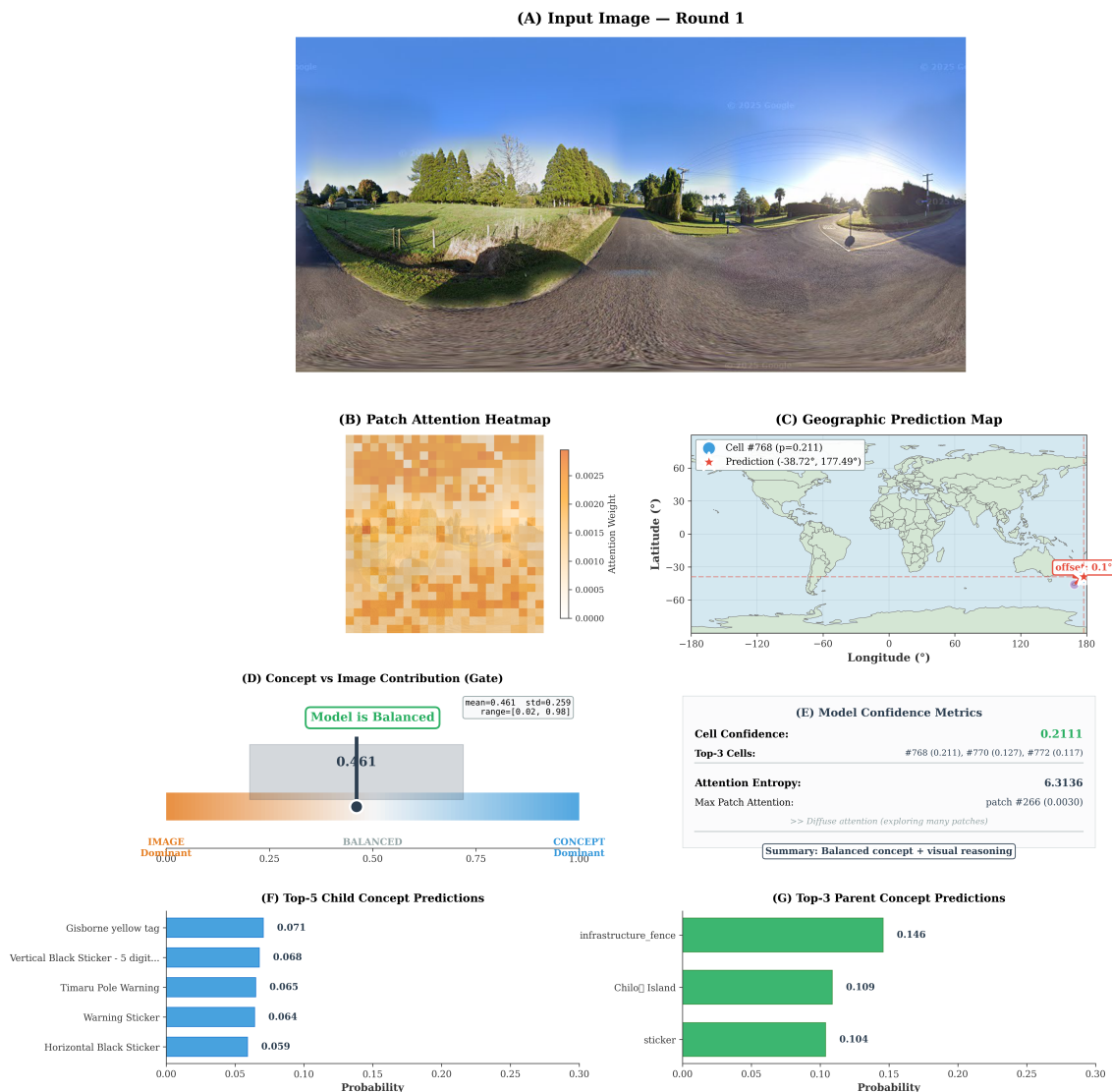
Figure 4: Interpretability analysis for Game 1 Round 1. This example demonstrates the model attending to architectural and infrastructure features for geolocation. The patch attention heatmap reveals focus on road geometry and built structures, while concept predictions capture semantic categories relevant to the predicted region.
