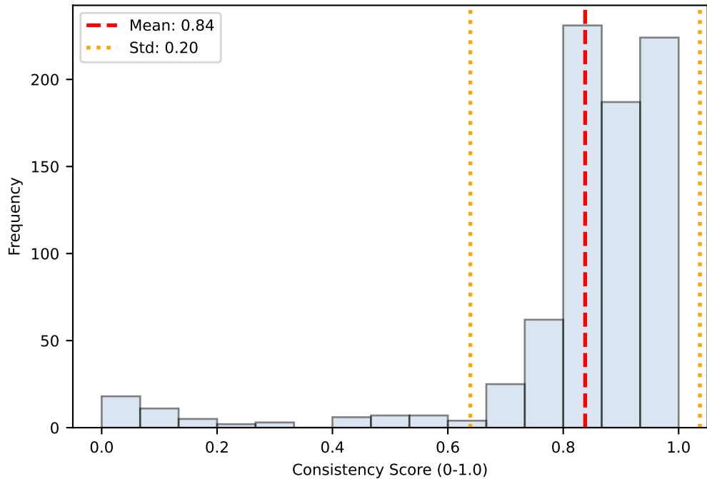
A: Bot Question Consistency (to Script)
