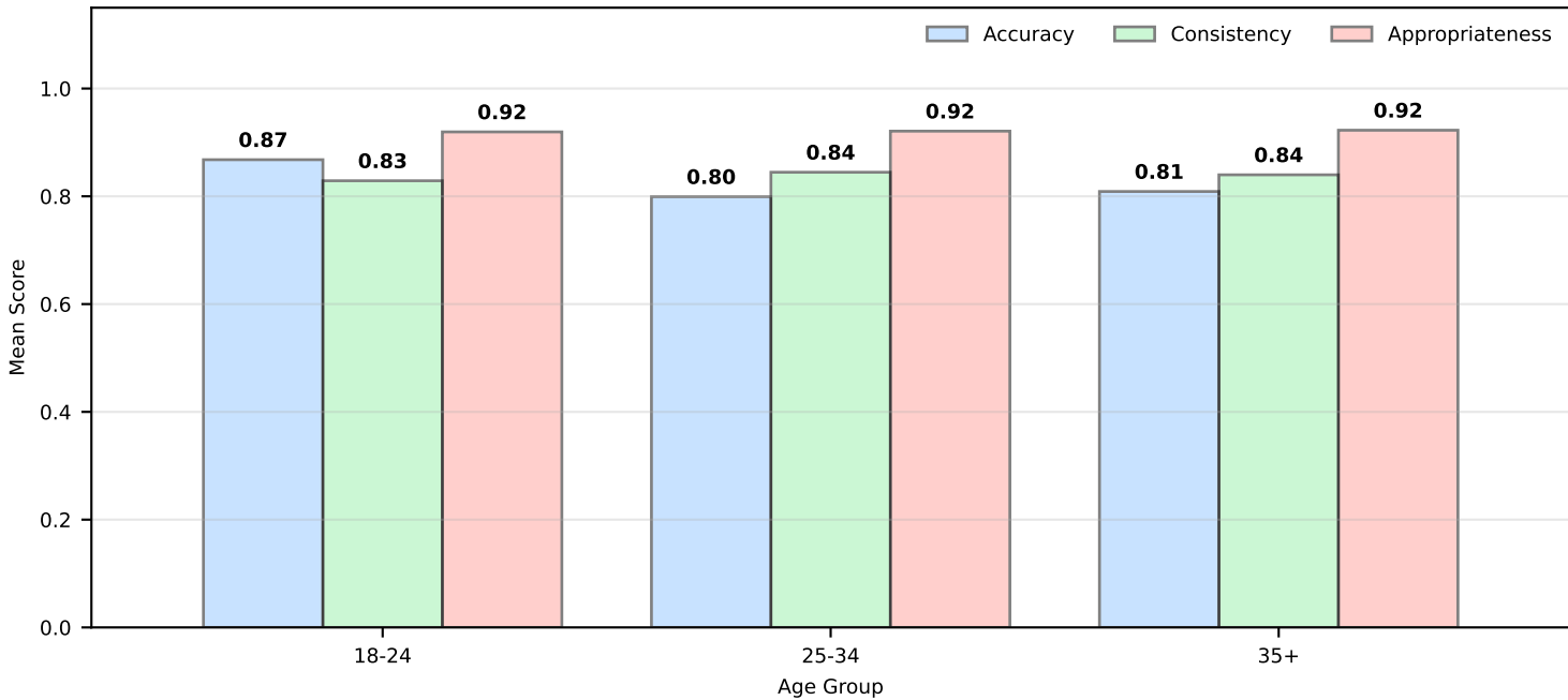
D: Detailed Performance by Age Group
