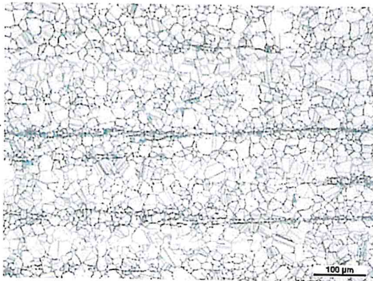
100:1 VDM® Alloy 625 /Nicrofer 6020 hMo SMT HCl - HNO 3 6:1 24.07.2024 11:02:48 101T002-A07 typical 1/4 thickness
