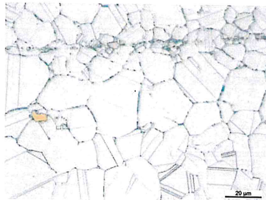
500:1 VDM® Alloy 625 /Nicrofer 6020 hMo SMT HCl - HNO 3 6:1 24.07.2024 11:02:49 101T002-A07 typical 1/4 thickness
