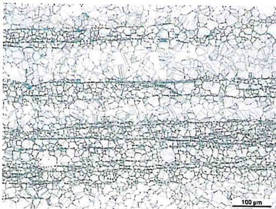
100:1 VDM® Alloy 625 /Nicrofer 6020 hMo SMT HCl - HNO 3 6:1 24.07.2024 11:02:51 101T002-A07 worst 1/4 thickness
