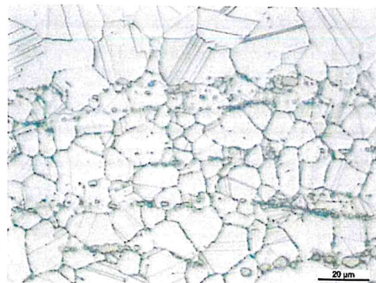
500:1 VDM® Alloy 625 /Nicrofer 6020 hMo SMT HCl - HNO 3 6:1 24.07.2024 11:02:52 101T002-A07 worst 1/4 thickness
