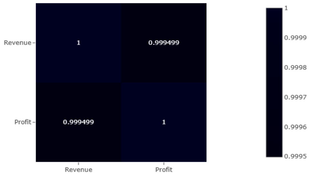
Correlation Heatmap
