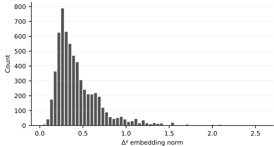
C4: Acceleration ( \Delta^2 ) norm
