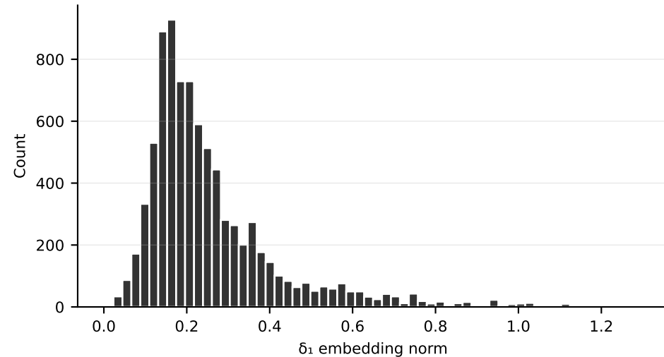
C4: Single-step visual delta ( \delta_1 ) norm
