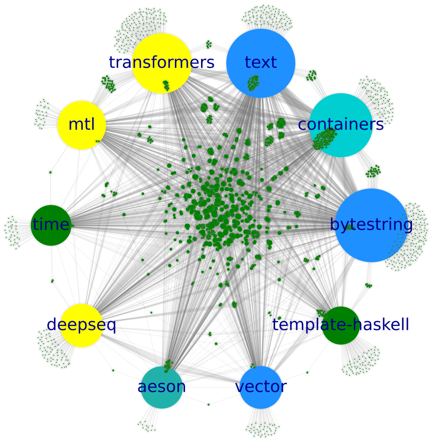
LTS 18-8
