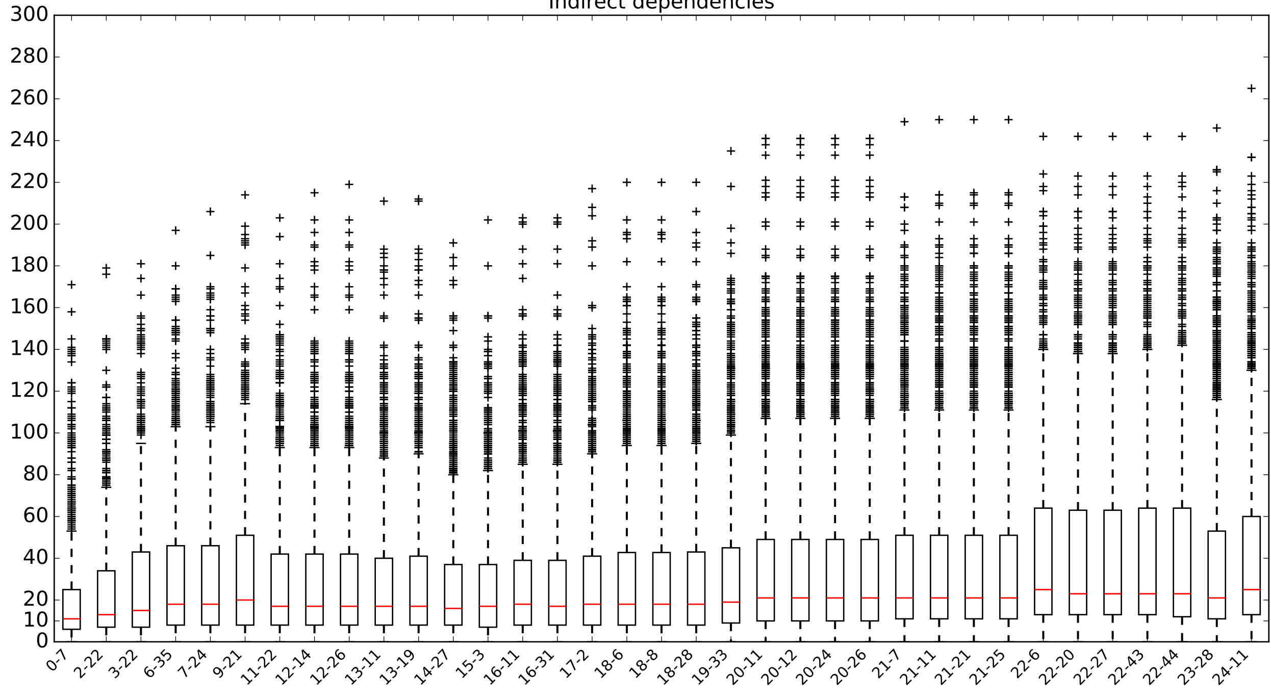
Indirect dependencies
