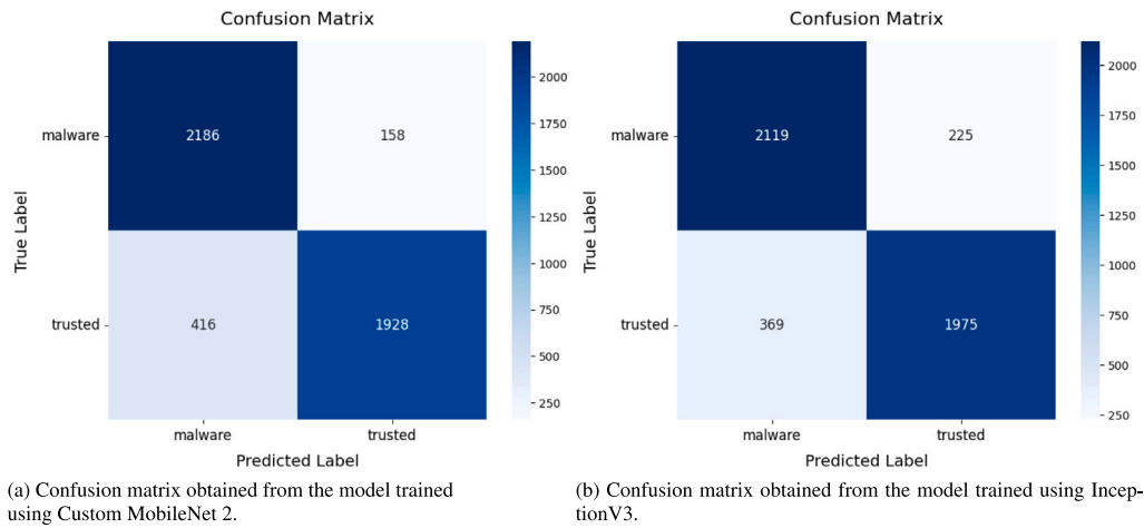
Fig. 7. Confusion matrices obtained after the test phase for the top-performing models: Custom MobileNet 2 (trained with CIFAR-10 weights) and Inception V3 (trained with ImageNet weights), evaluated using Clipping Norm Aggregator and on IID data.
