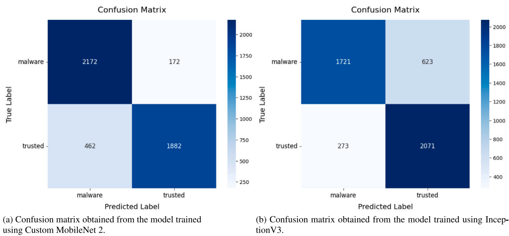
Fig. 9. Confusion matrices obtained after the test phase for the top-performing models: Custom MobileNet 2 (trained with CIFAR-10 weights) and Inception V3 (trained with ImageNet weights), evaluated using Clipping Norm Aggregator and on non-IID data.
