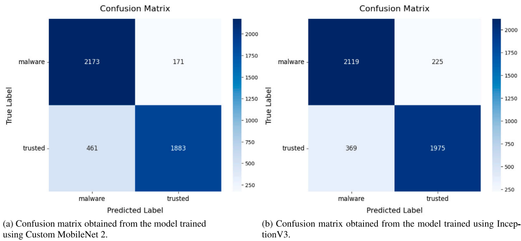
Fig. 8. Confusion matrices obtained after the test phase for the top-performing models: Custom MobileNet 2 (trained with CIFAR-10 weights) and Inception V3 (trained with ImageNet weights), evaluated without normalization and on non-IID data.
