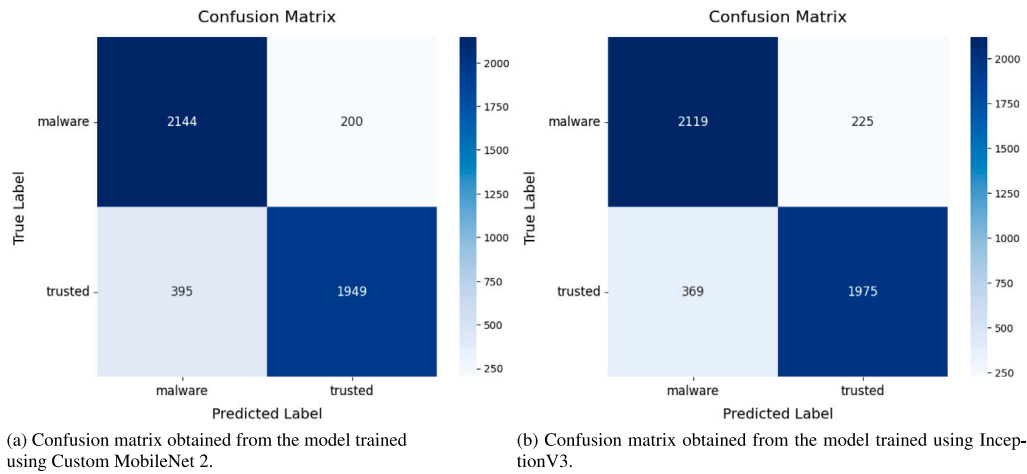
Fig. 6. Confusion matrices obtained after the test phase for the top-performing models: Custom MobileNet 2 (trained with CIFAR-10 weights) and Inception V3 (trained with ImageNet weights), evaluated without normalization and on IID data.
