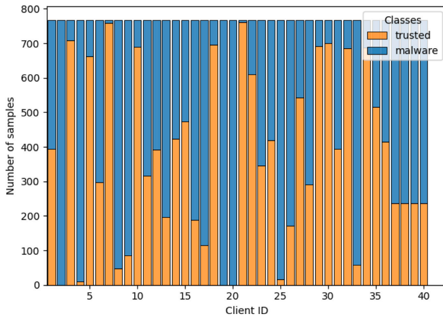
Fig. 4. The Dirichlet distribution obtained among 40 different clients.
