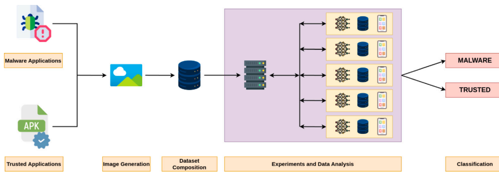
Fig. 1. The workflow of the proposed privacy-preserving Android malware detector.
