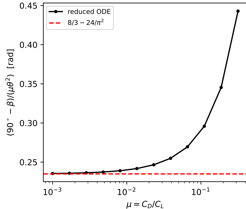
asymptotics as \mu \rightarrow 0
