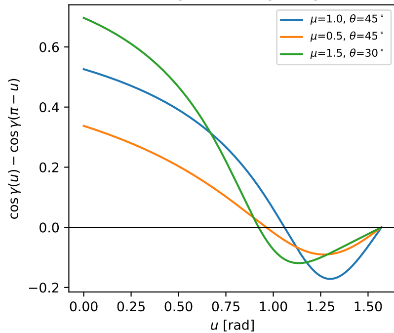
folded integrand changes sign once
