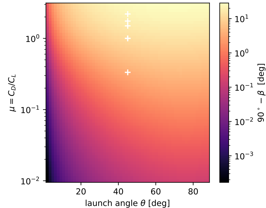
chord-bearing deficit (always > 0 )
