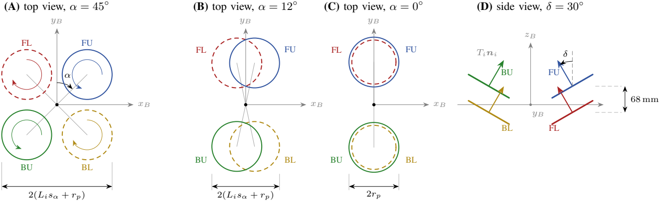
Fig. 2. Morphing geometry and dihedral tilt. (A) X configuration, with rotor colors denoting FU, FL, BU, and BL. L_i is the length of an arm, r_p is radius of propeller; upper rotors are solid and lower rotors dashed. (B) During morphing, the rotor pairs converge and the lateral moment arm shrinks with L_i \sin \alpha . (C) At \alpha = 0^\circ , the front and rear rotor pairs overlap along y_B . (D) The motors use a fixed dihedral \delta = 30^\circ . Relative to the center of gravity, the upper and lower rotor planes are located at z_U = +48 mm and z_L = -20 mm, giving a vertical separation of 68 mm.
