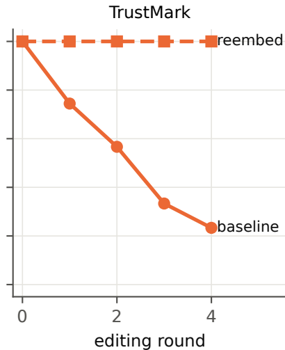
Baseline vs watermark-aware methods (InstructPix2Pix)
