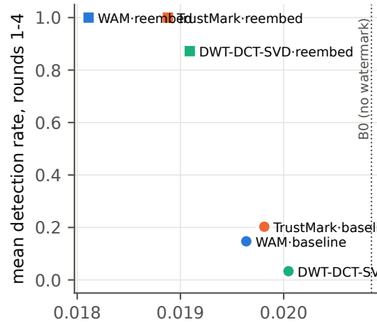
flux2klein
