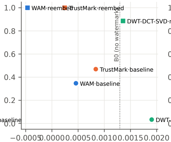
InstructPix2Pix
