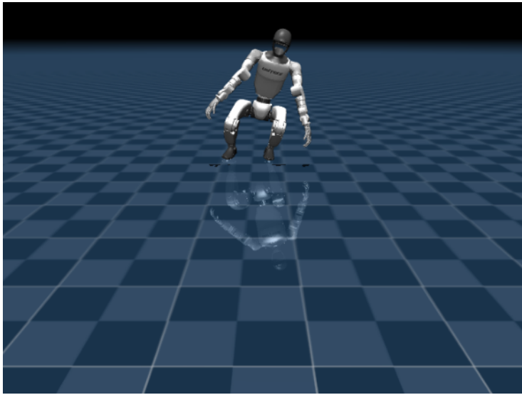
B 120 N push: CP escaping support
