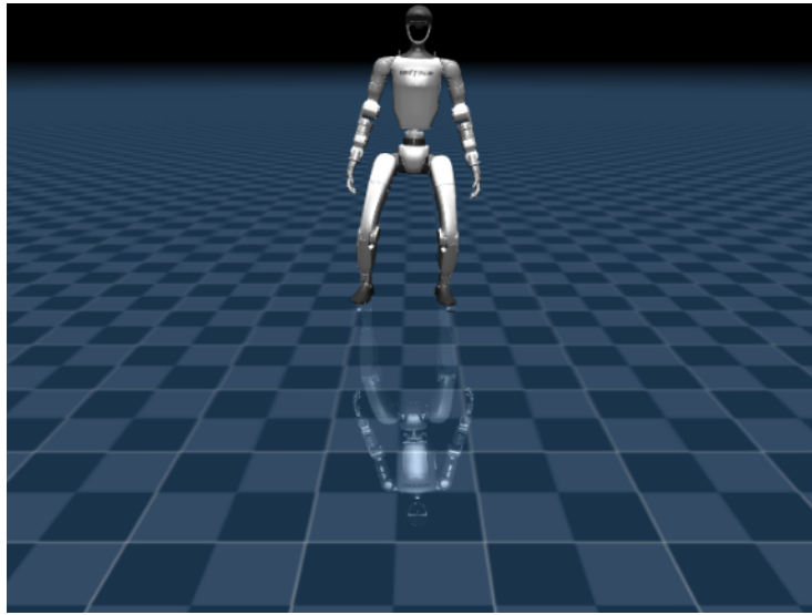
C 100 N push: CP held inside
