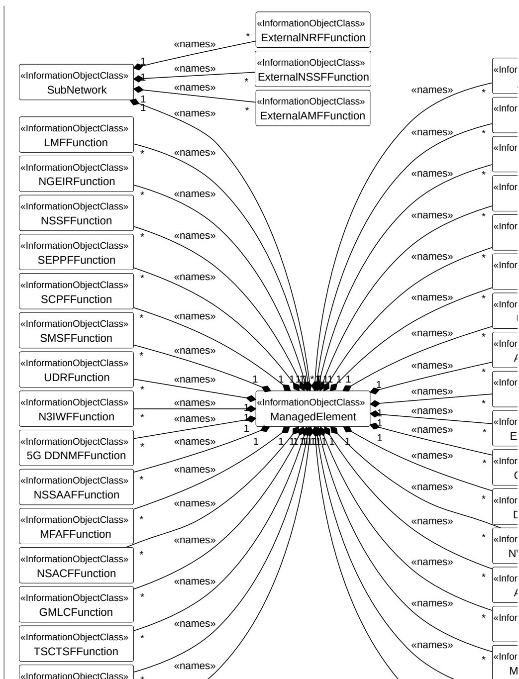
Figure 5.2.1.1-1: 5GC NRM containment/naming relationship
