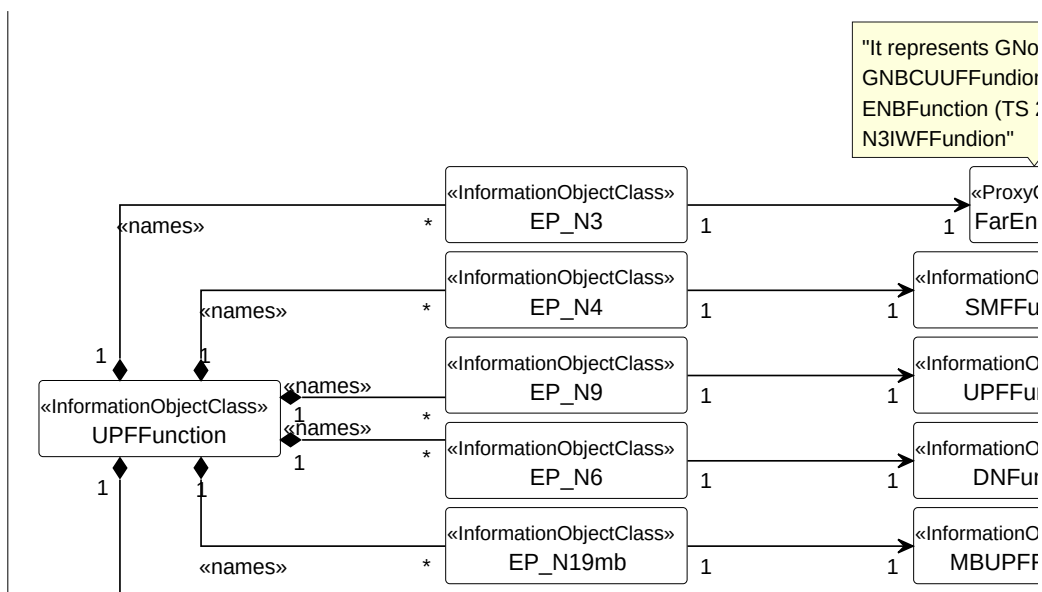
Figure 5.2.1.1-4: Transport view of UPF NRM
