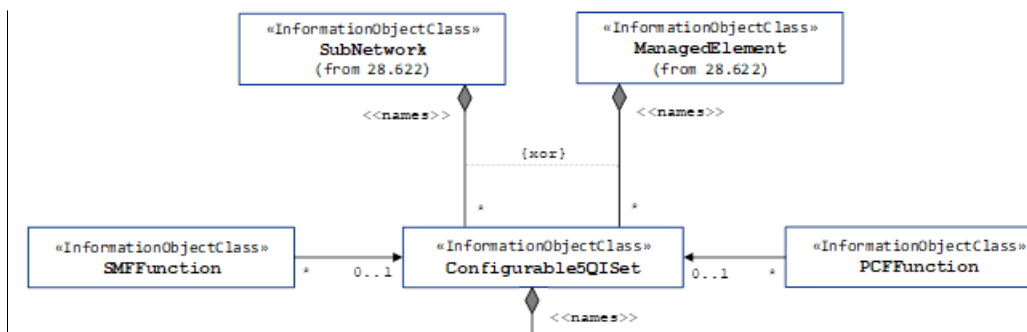
Figure 5.2.1.1-17: NRM fragment for pre-configured 5QIs in 5GC
