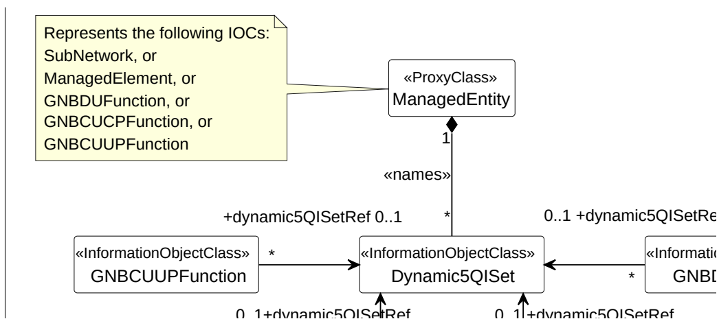
Figure 4.2.1.1-16: NRM fragment for dynamically assigned 5QIs in NG-RAN
