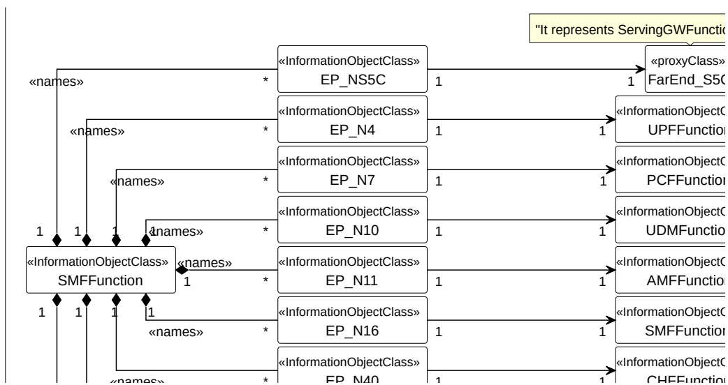
Figure 5.2.1.1-3: Transport view of SMF NRM
