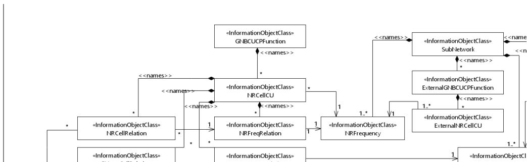
Figure 4.2.1.1-4: Cell Relation view for all deployment scenarios
