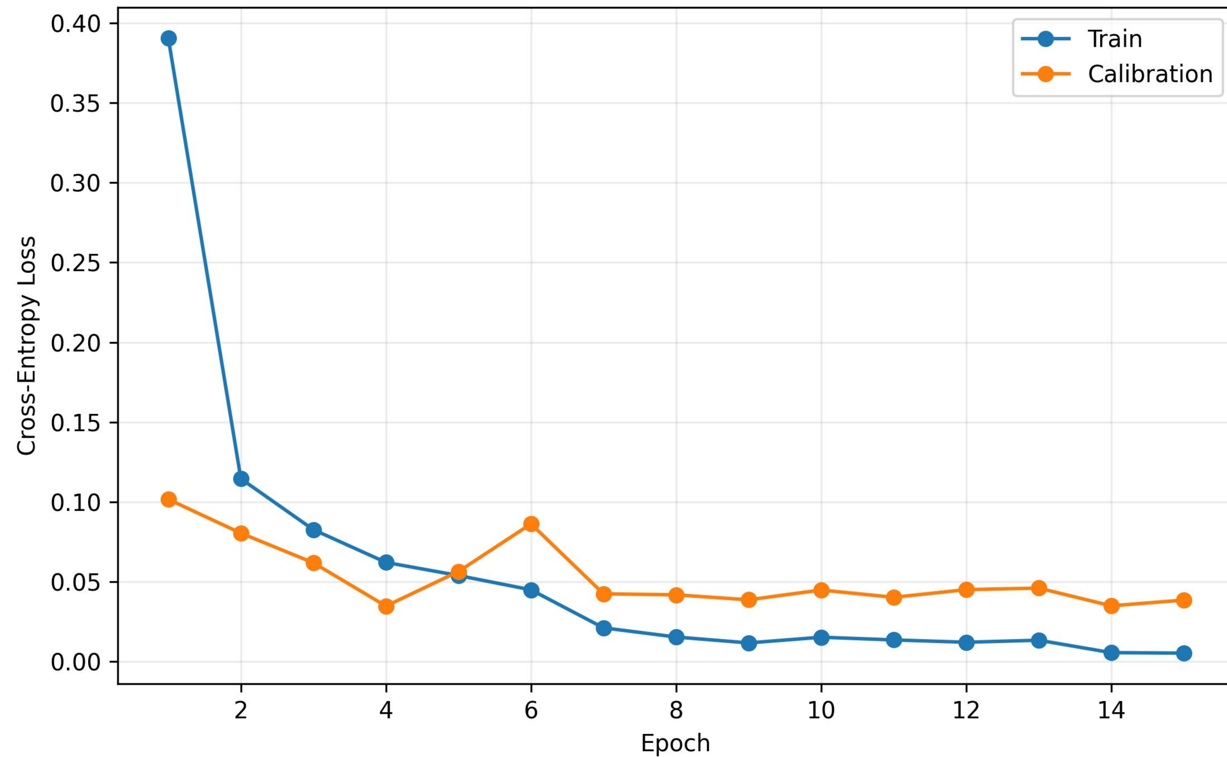
Loss by Epoch
