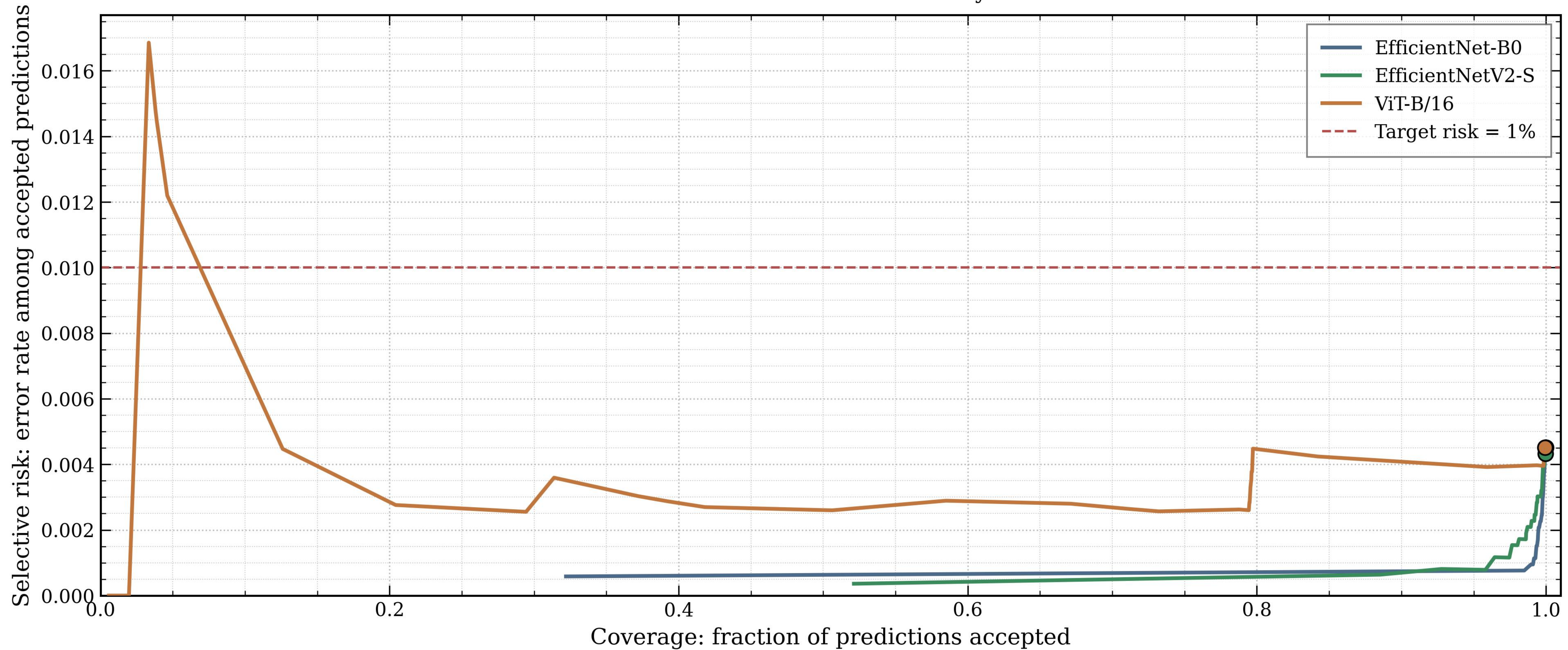
Internal-test risk-coverage curves Markers indicate thresholds chosen exclusively on calibration data
