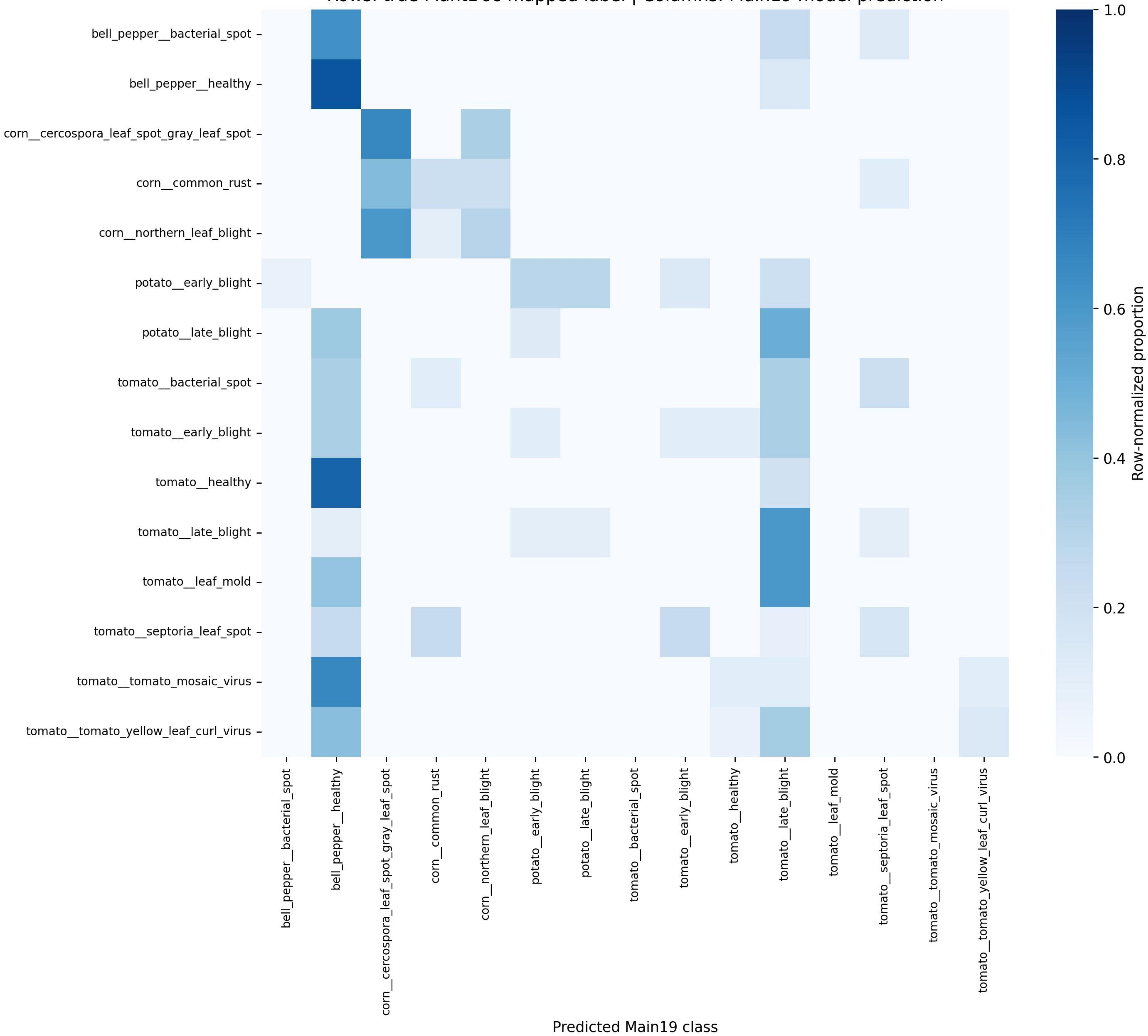
PlantDoc external-domain confusion matrix Rows: true PlantDoc-mapped label | Columns: Main19 model prediction
