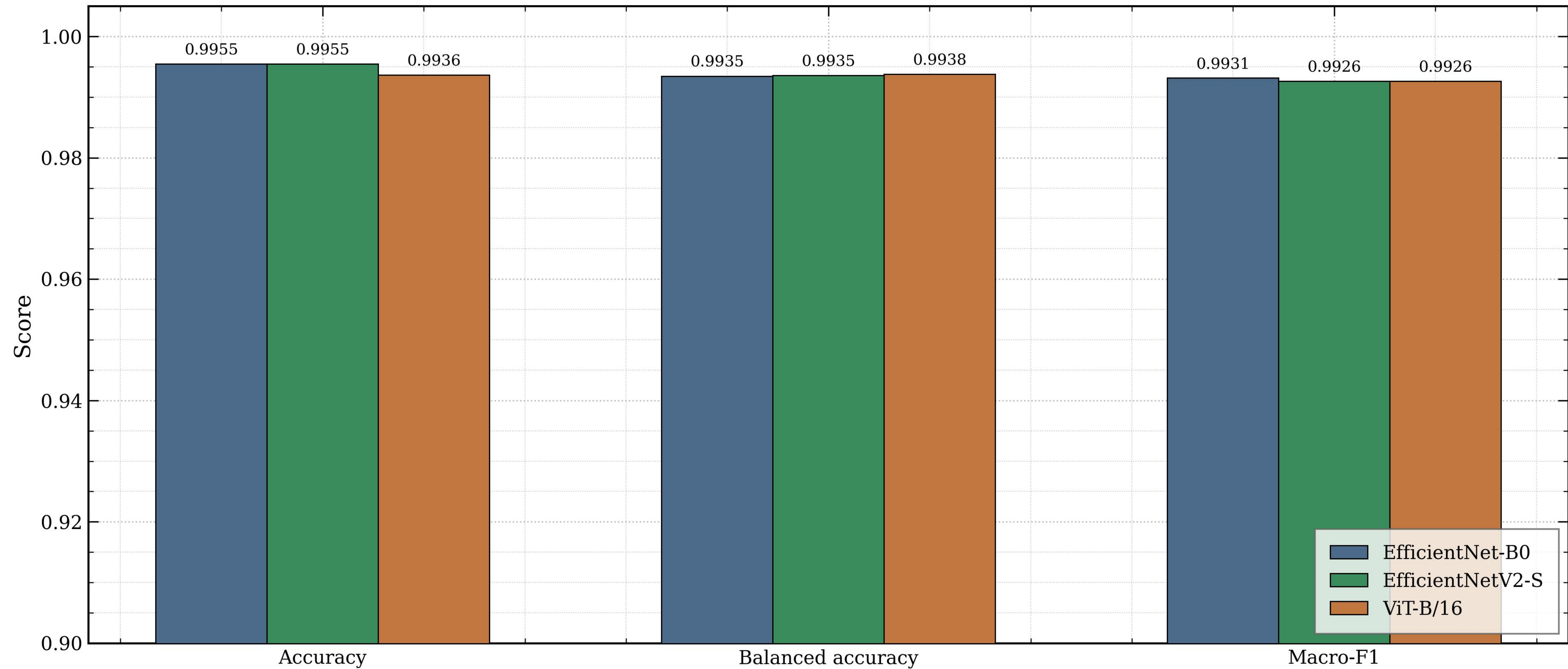
CNN versus Vision Transformer performance on Main19 internal test
