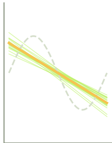
degree 1
