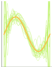
degree 15
