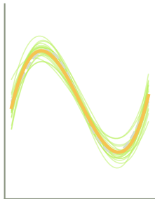
degree 3
