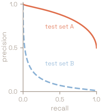
precision-recall
