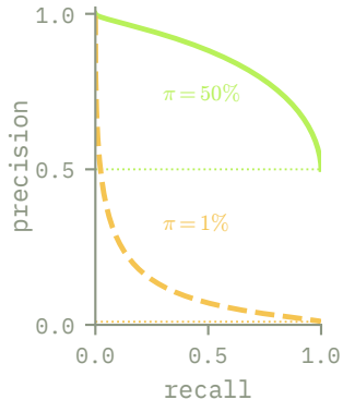
precision-recall
