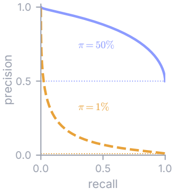
precision-recall
