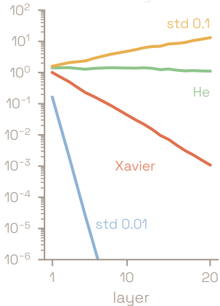
ReLU layers
