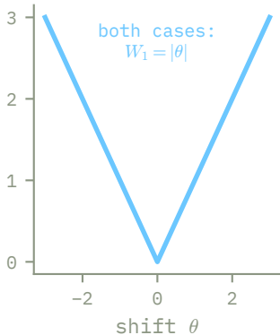
W_1 distance
