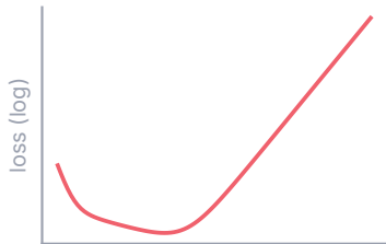
C: overfitting
