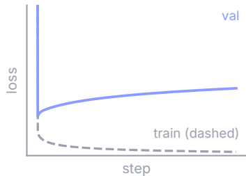
C: overfitting
