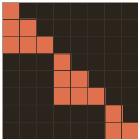
causal + document mask
