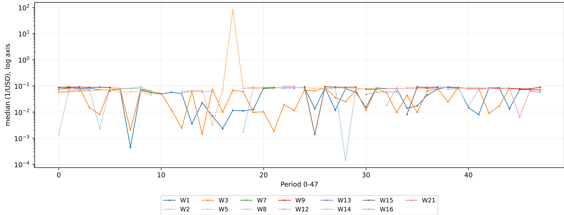
Median M10 epsilon by 30-minute Period and WeatherCode
