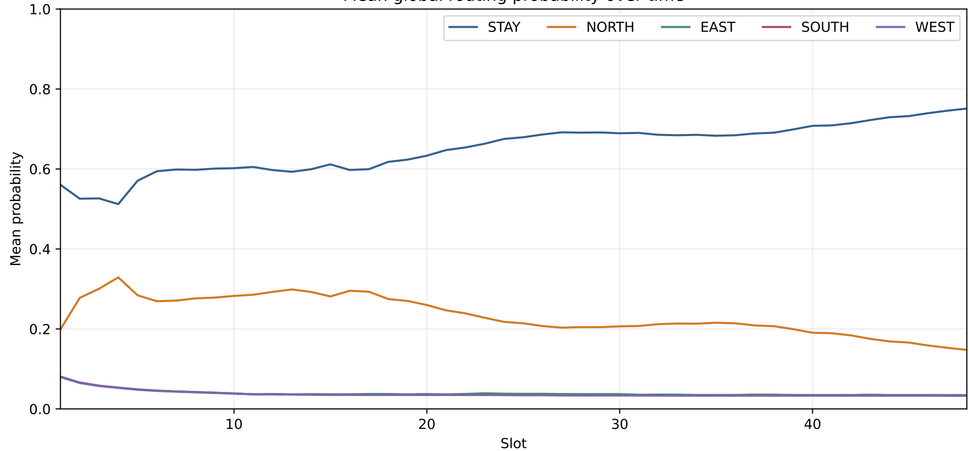
Mean global routing probability over time
