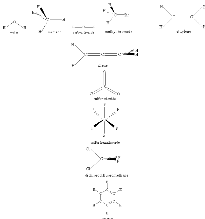
Figure 3.2: Molecules of Study originally listed in Table 4.1.
