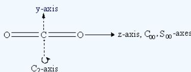
Figure 3.9: Symmetry elements of carbon dioxide
