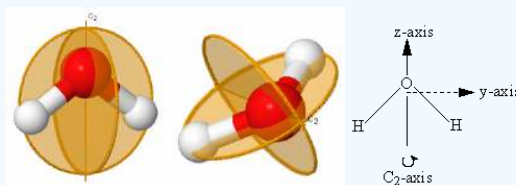
Figure 3.8: Symmetry elements of water viewed from differing perspectives
