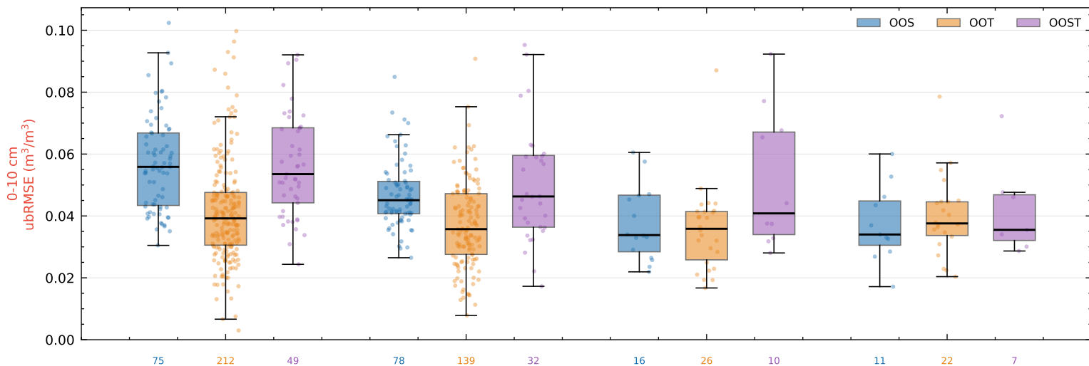
Per-station ubRMSE by igbp_macro and split
