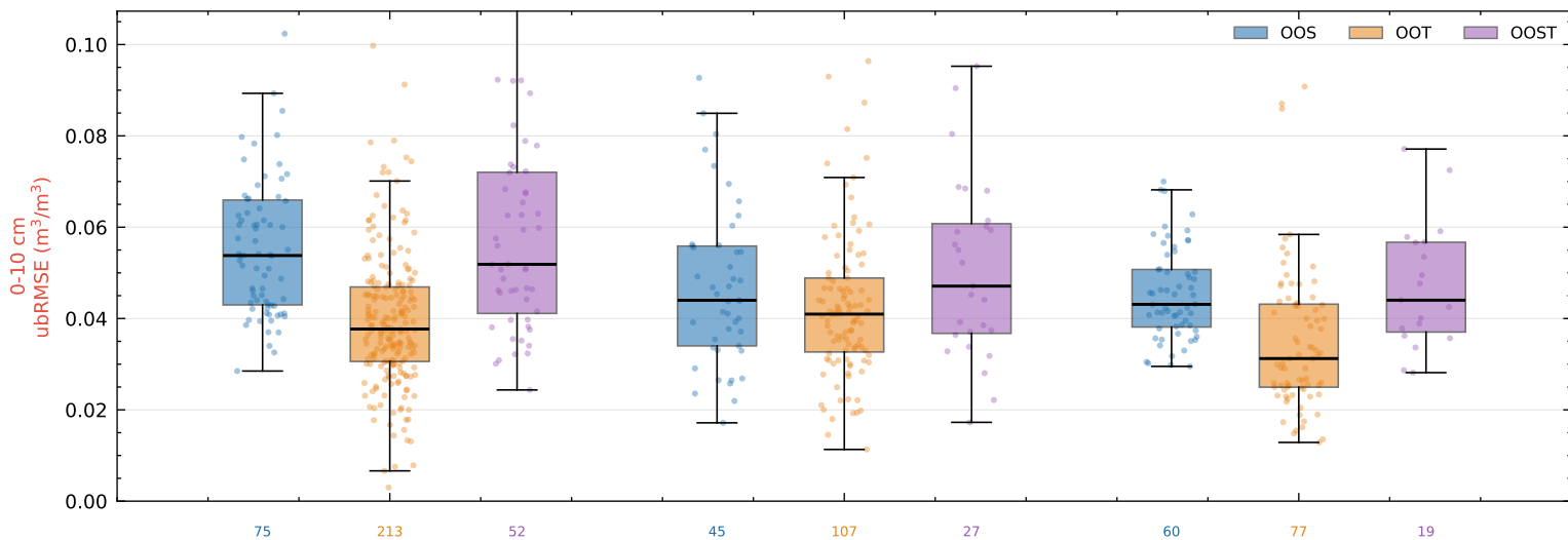
Per-station ubRMSE by kg_macro and split
