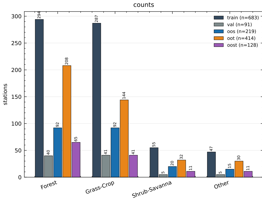
Station inventory by igbp_macro -- train vs held-out splits
